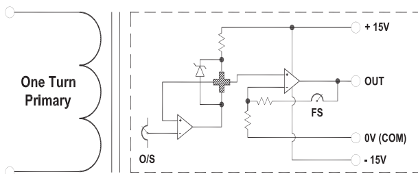
SCHEMATIC
